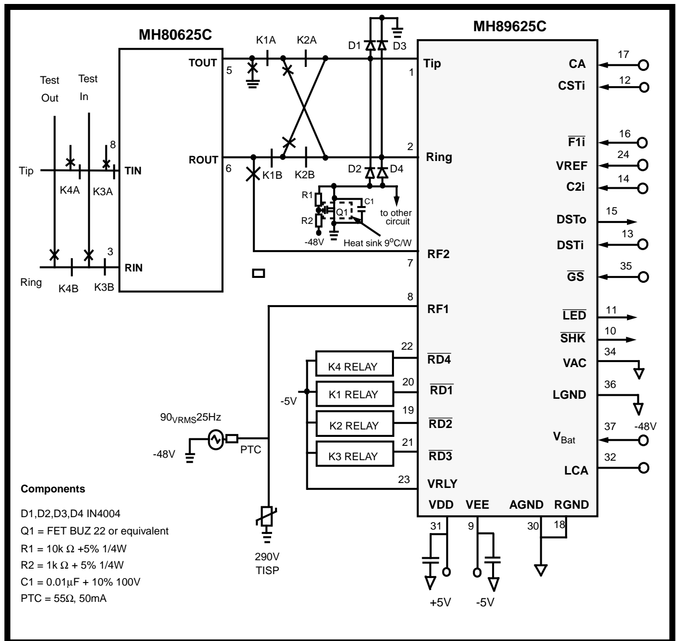
Figure 3 - Typical Line Card Application
