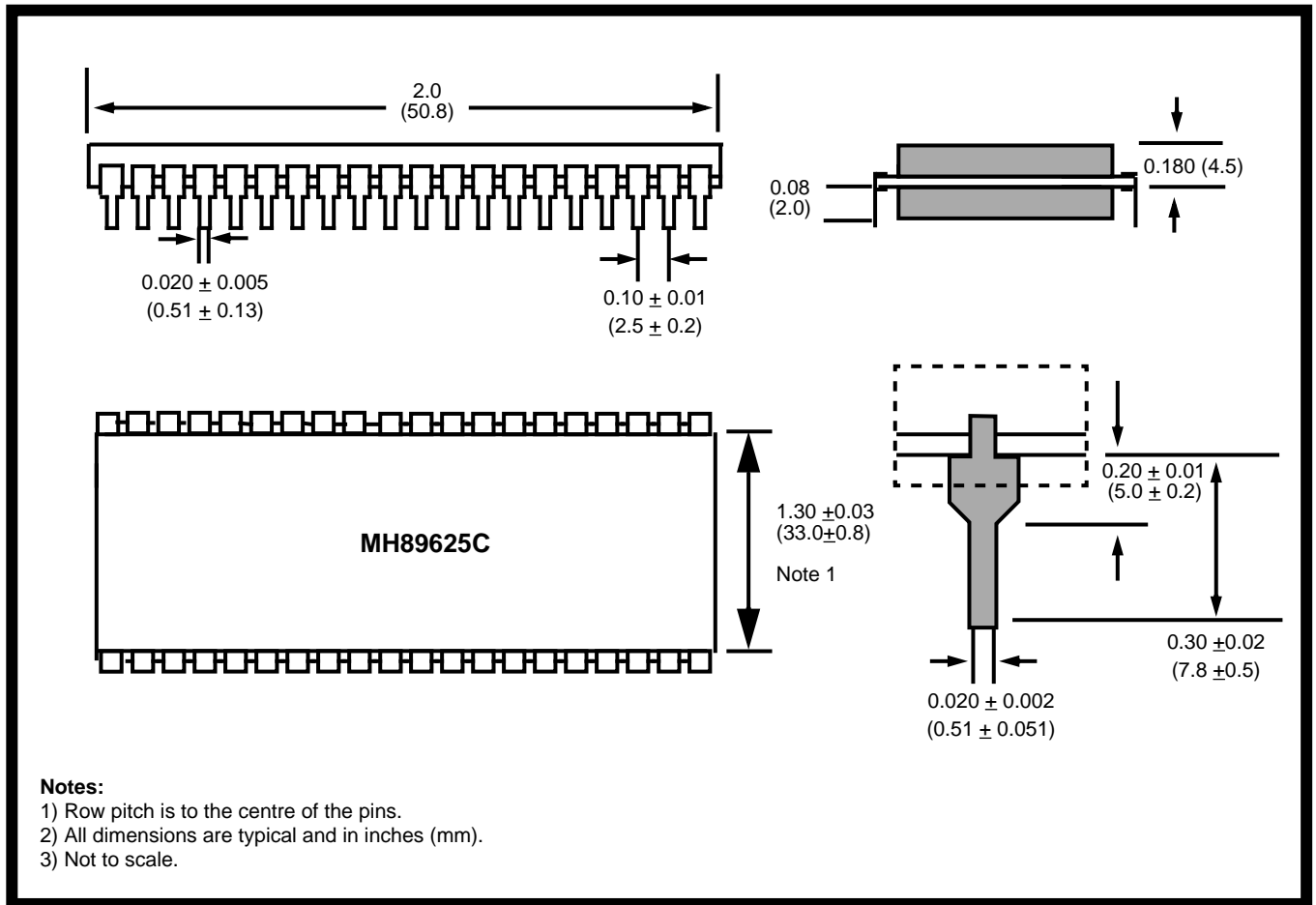
Figure 6 - Mechanical Data
